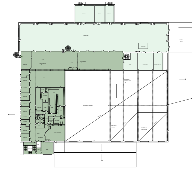
PLAN 1
